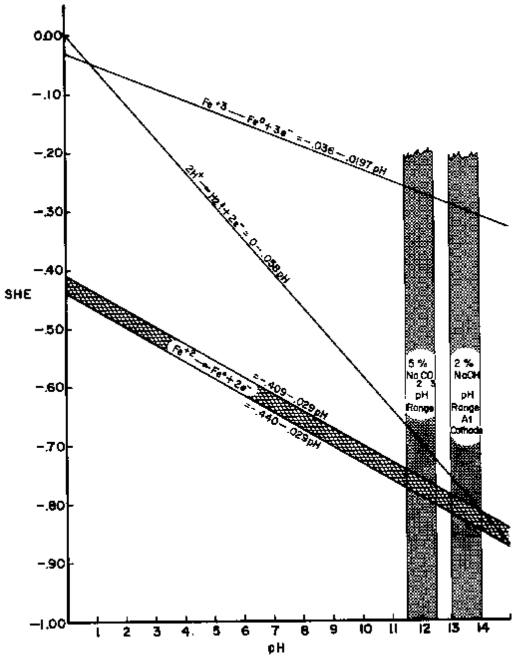
Figure 6. Reduction Potentials of Ferric, Ferrous, and Hydrogen Ions at Different pH's and Standard Temperature of 20 °C. The pH Range of a 5% \text{Na}_2\text{CO}_3 and a 2% \text{NaOH} Electrolyte are shaded.
